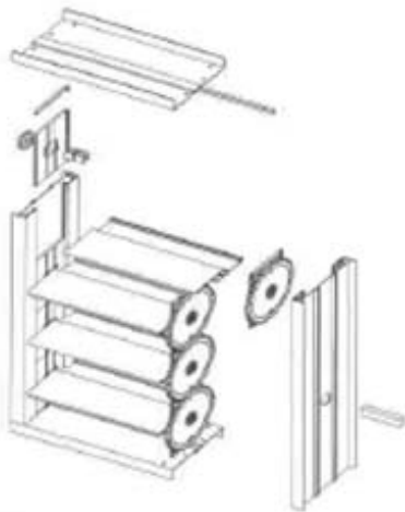
Single Damper assembling scheme
